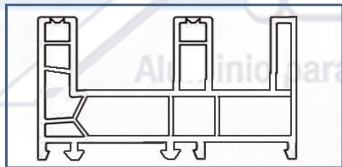
Contramarco Ventana Corrediza 88mm ( T88-PK(J) )
