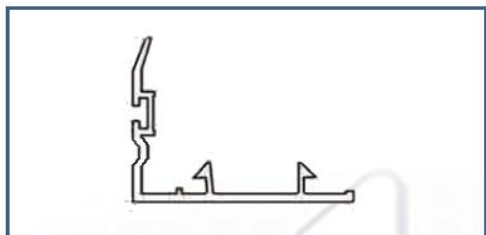
Traslape Ventana Corrediza 95mm (T95-FB)
