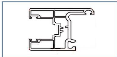
Hoja Ventana Corrediza 95mm (T95-S)
